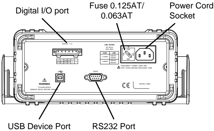
DIGITAL I/O
